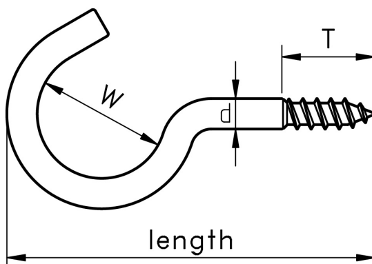
Figure 1: Cup Hook with Wood Thread
