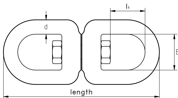
Figure 1: Swivel Shackle with Eyes
