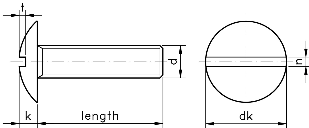
Figure 1: Slotted Mushroom Head Screw
