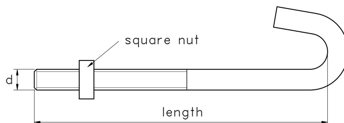
Figure 1: J Hook and Nut Bolt
