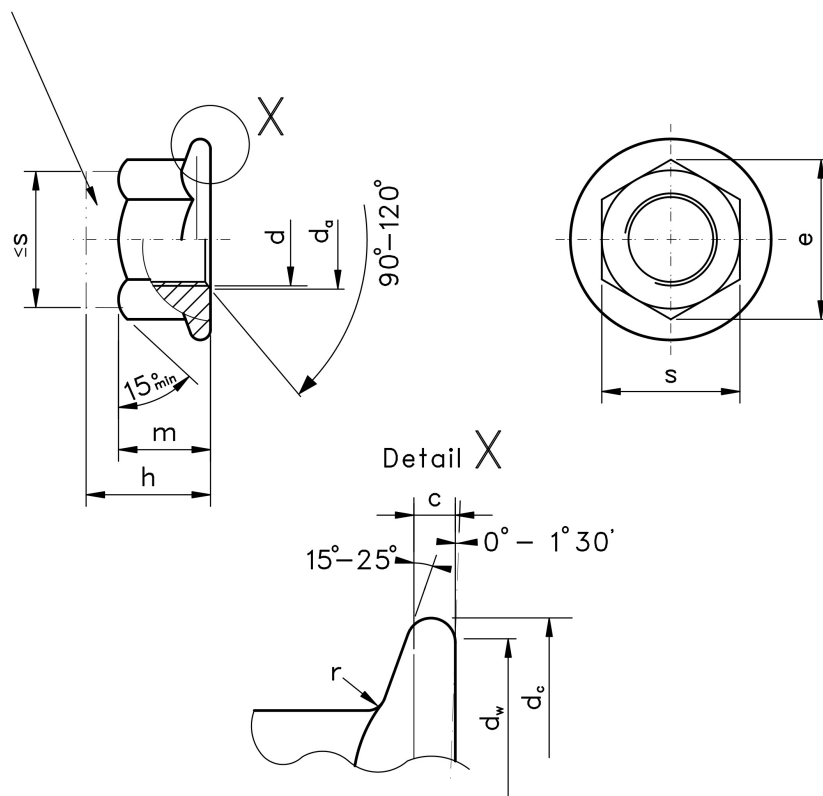
Figure 1: Hex Plain (Non-Serrated) Flange Nut with Nylon Insert
