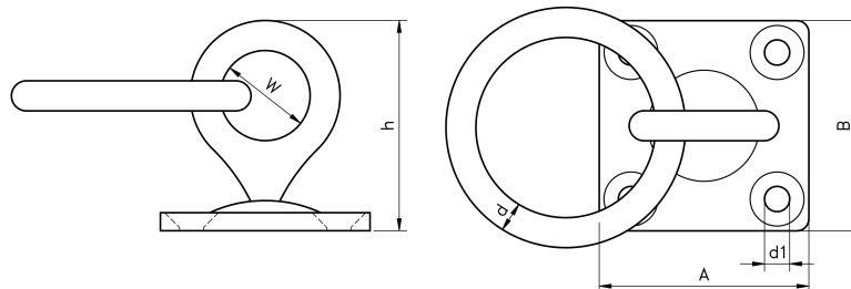
Figure 1: Square Pad Eye with Swivel & Ring
