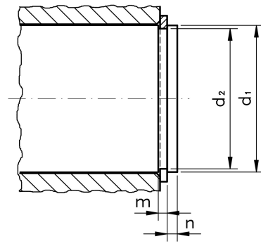
Figure 2: External Circlip, Sectional View of Fitment
