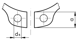
Figure 1: External Circlip, General Layout
