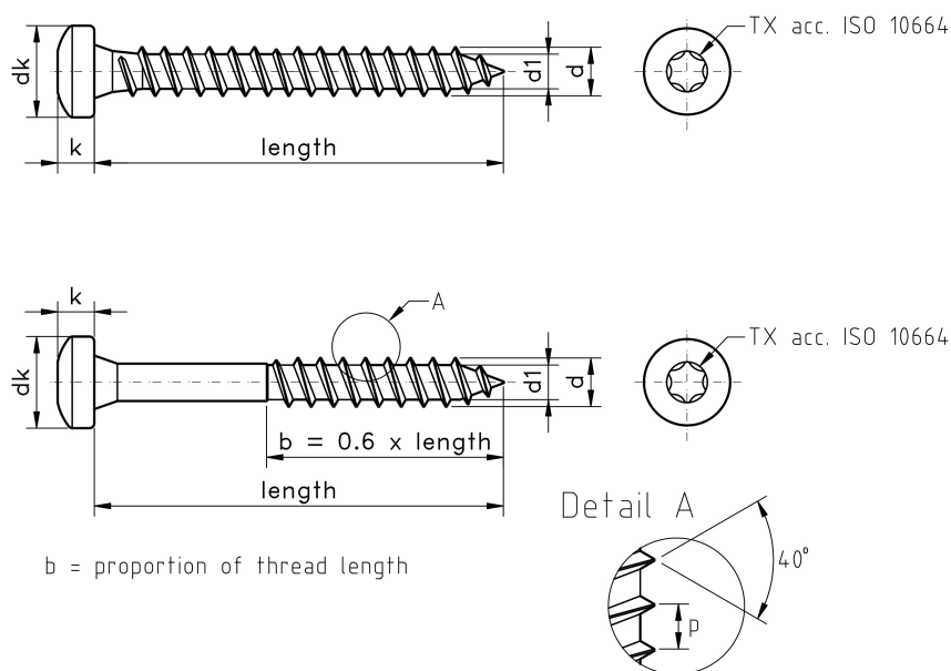
Figure 1: Torx Pan Head Chipboard Screw
