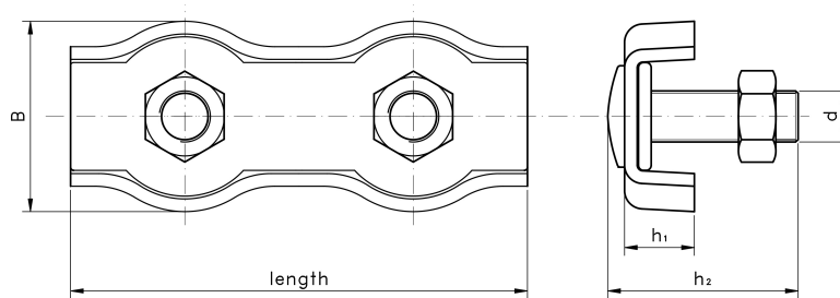
Figure 1: Wire Clamp, Duplex Type
